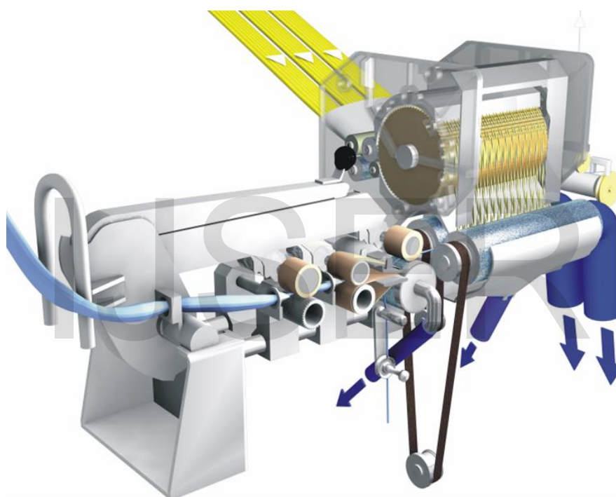
Fig. 4. Dref 3000 Spinning Machine
